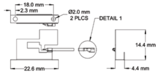
Detail 1 shows correct cable and connector orientation
